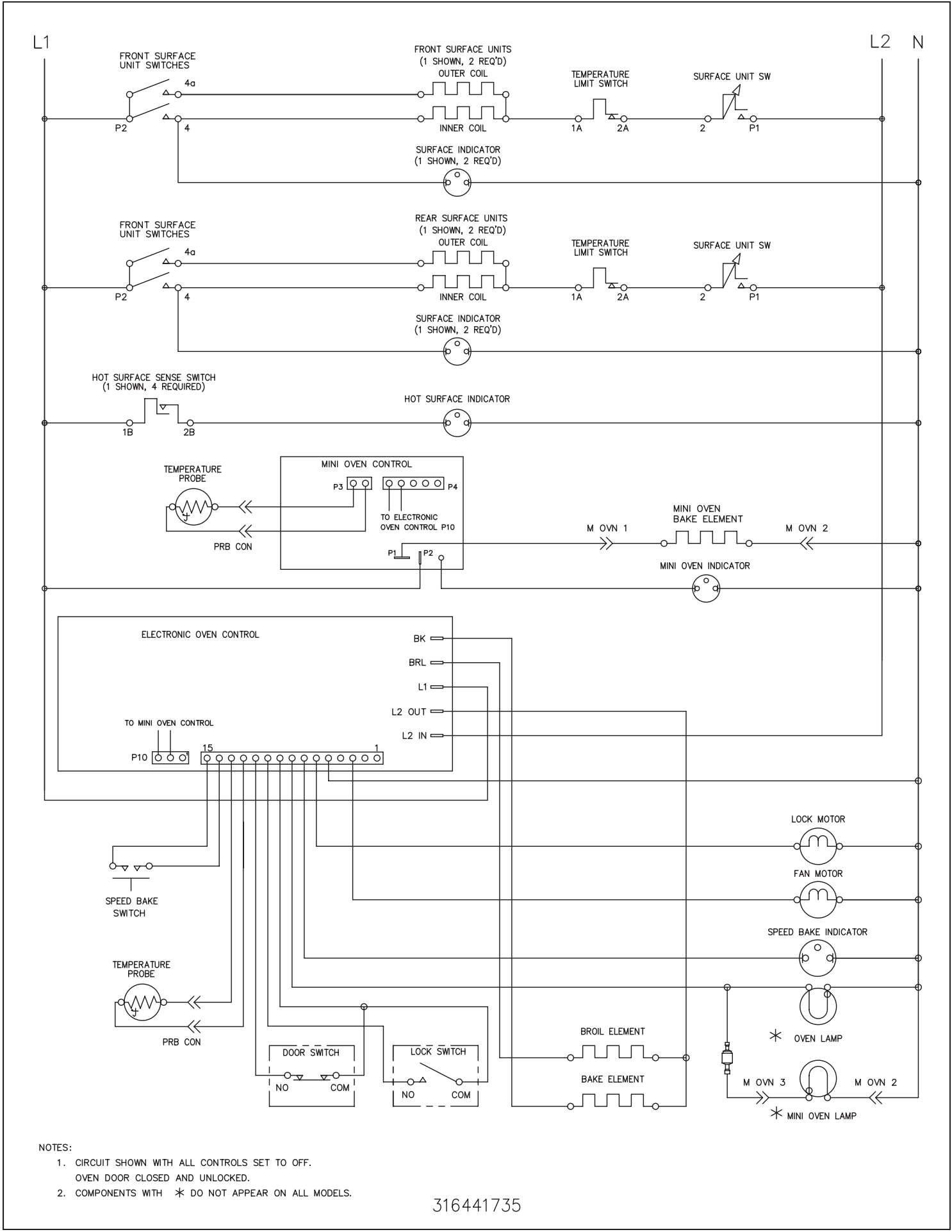
General Troubleshooting Schematic
