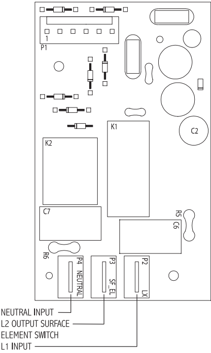
Simmer Select PCB (some models)
