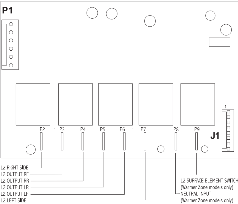
Cooktop Lockout PCB (some models)
