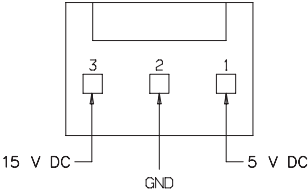
P10 Bake-N-Warm™ Double Oven Connection (some models)
