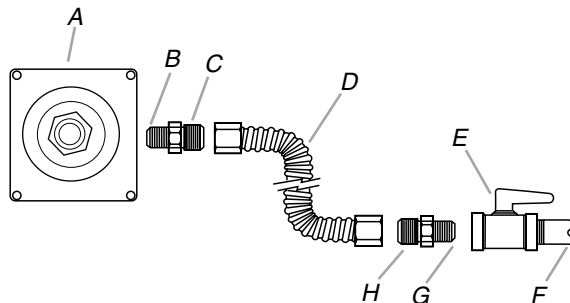
A. Gas pressure regulator B. Use pipe-joint compound. C. Adapter (must have \frac{1}{2} " male pipe thread) D. Flexible connector
