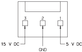
EOC P10 BAKE-N-WARM™ CONNECTION (some models)
