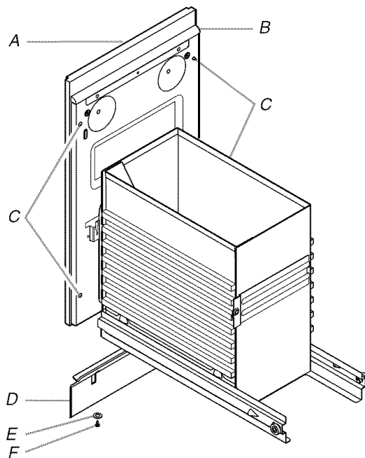
A. Custom panel B. 15" x ½" quarter-round C. Panel screw locations D. Toe guard E. Washer F. Toe guard screw
