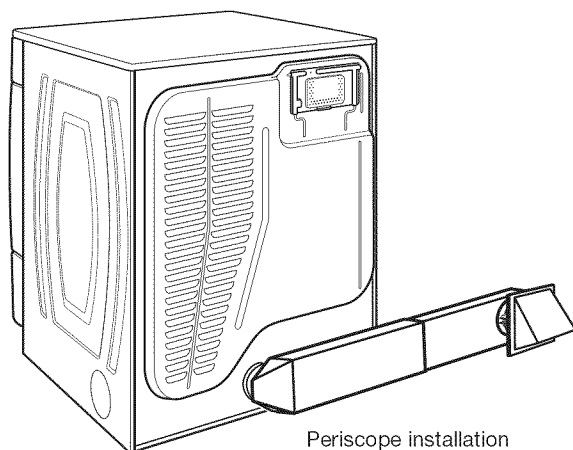
Periscope installation
