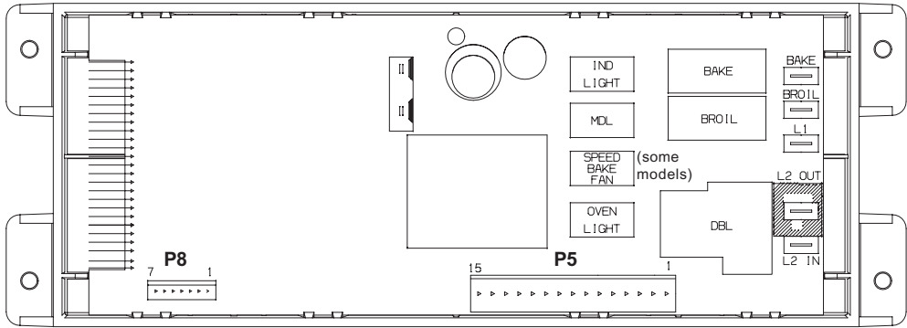
P8 Cooktop Lockout Connections (some models)
