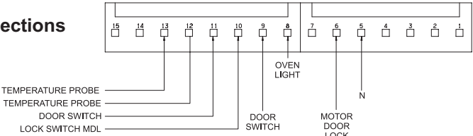
P8 Cooktop Lockout Connections (some models)
