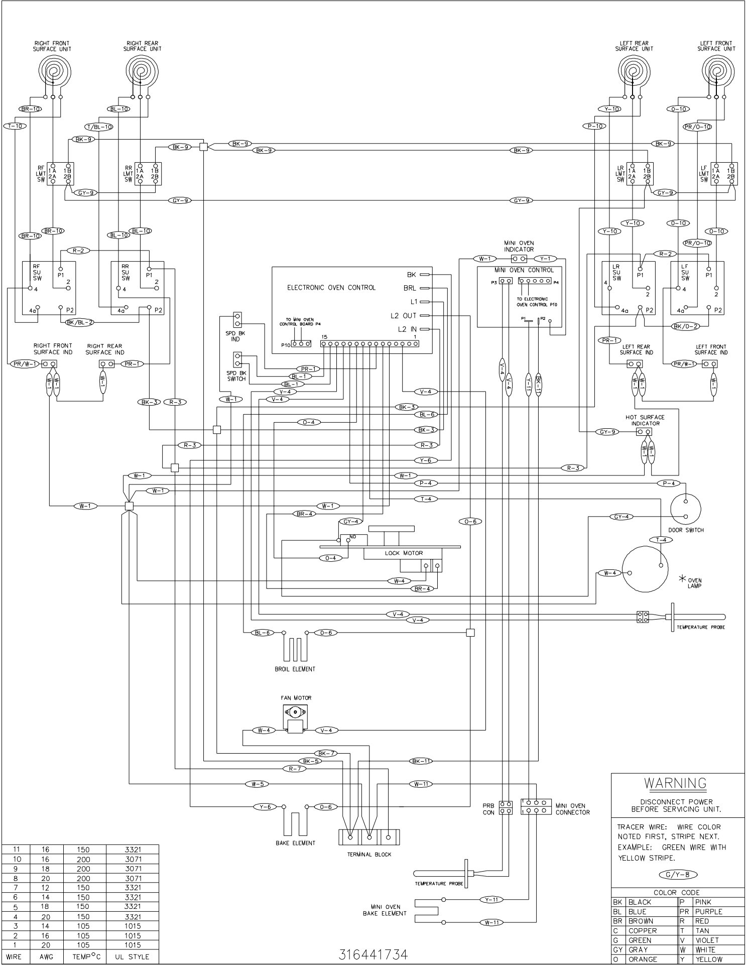
Genral Troubleshooting Wiring Diagram
