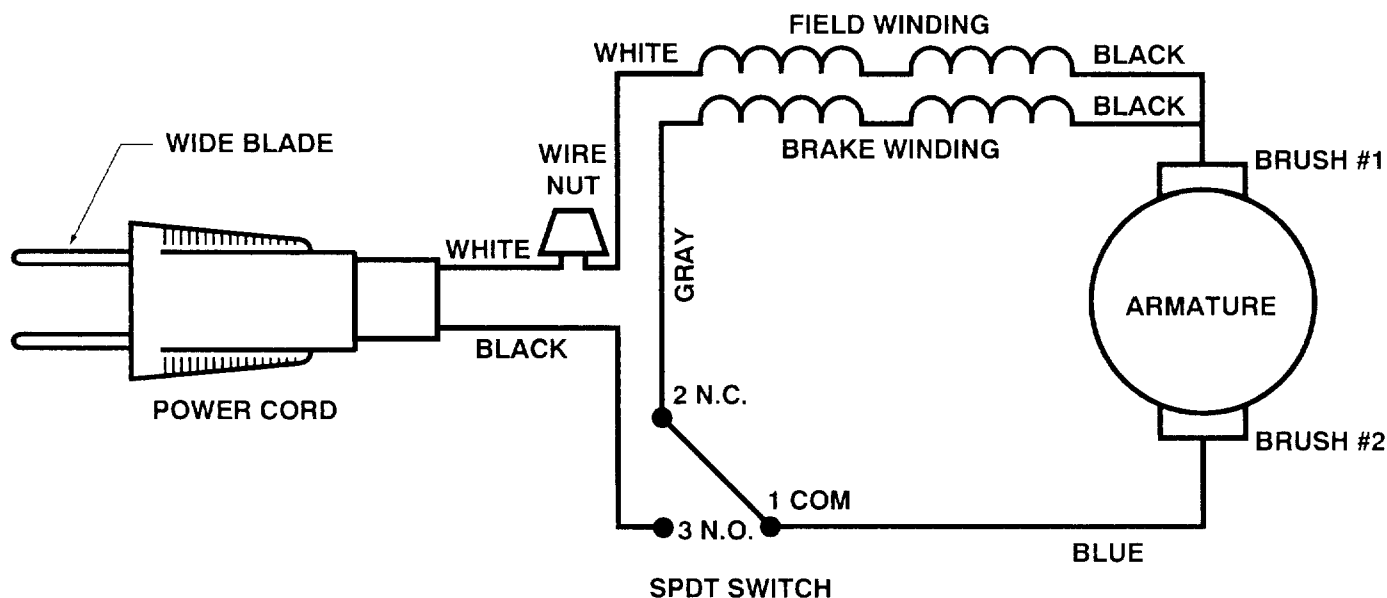
Circuit Diagram
