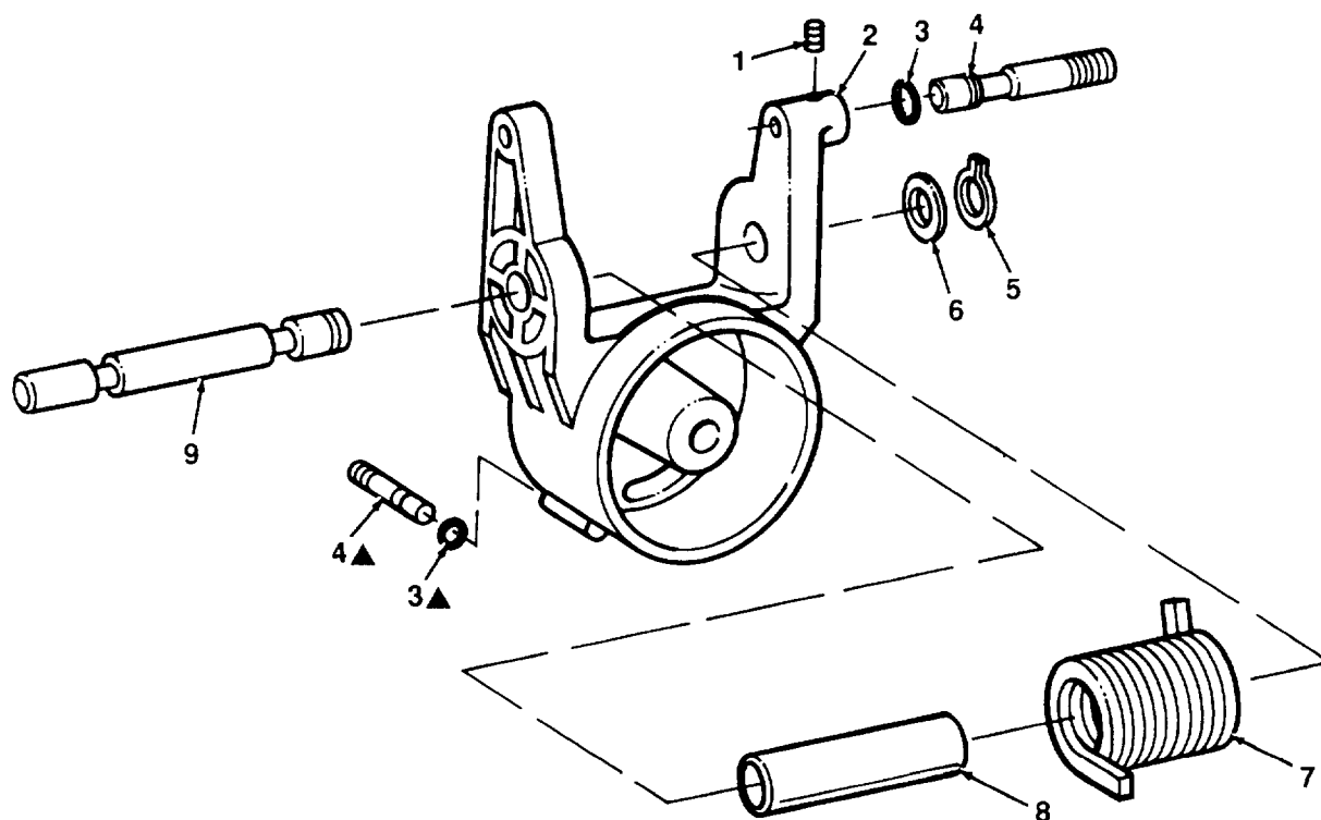
FIGURE 3—PIVOT ASSEMBLY
