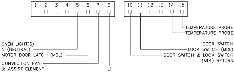
EOC P5 CONNECTIONS
