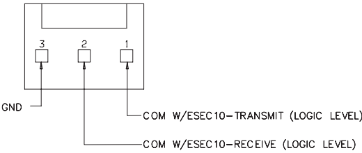
EOC P4 BAKE-N-WARM™ CONNECTION (some models)
