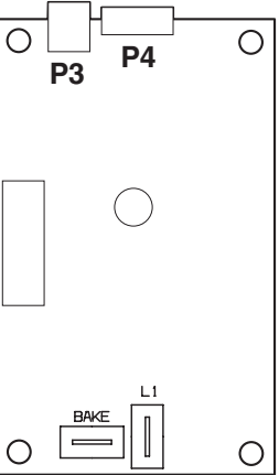
BAKE-N-WARM™ DOUBLE OVEN CONTROL BOARD (REAR VIEW)
