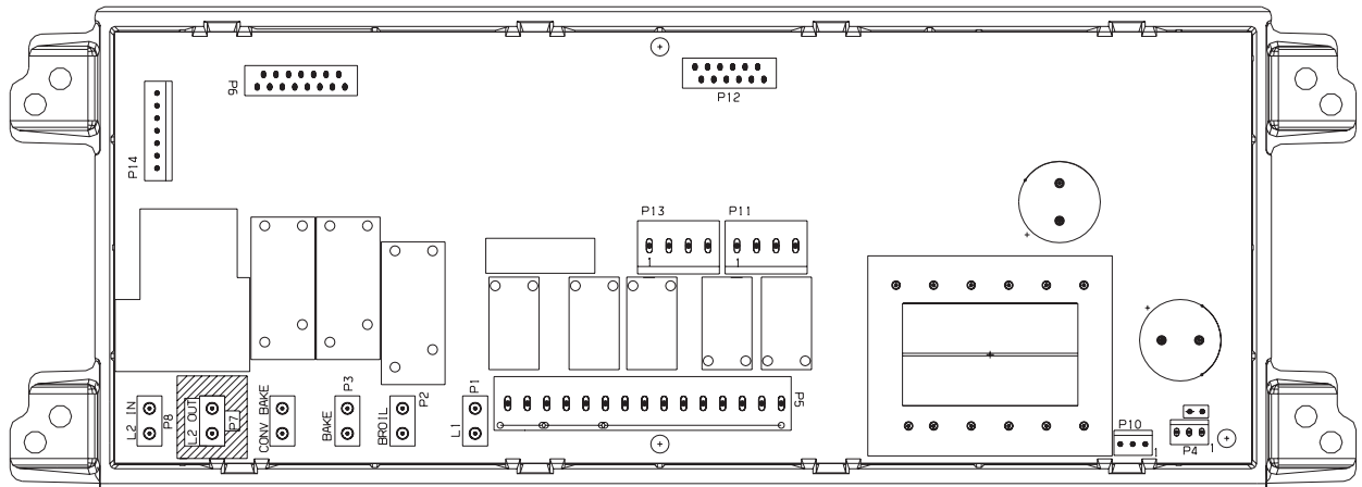
EOC P10 BAKE-N-WARM™ CONNECTION (some models)
