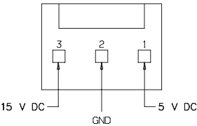
EOC P10 BAKE-N-WARM™ CONNECTION (some models)
