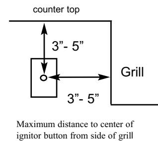
Built-in dimensions using a Trim Kit
