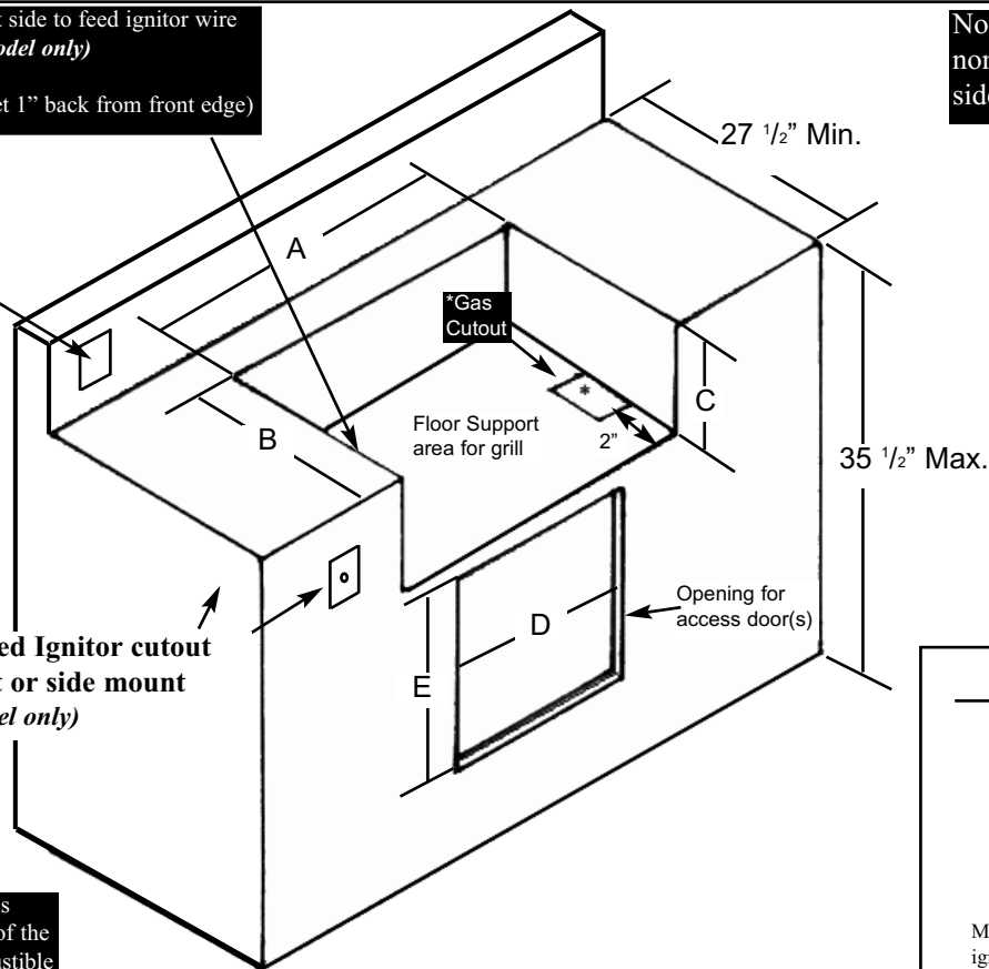
Built-in dimensions without using a Trim Kit
