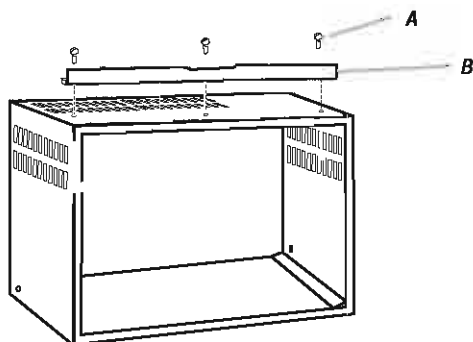
A. Top channel B. #10 x 3/8" pan-head Phillips thread-cutting screws
