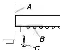
A. Window channel B. Left-hand curtain C. #10 x \frac{3}{4} " round-head screw
