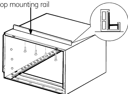
Top mounting rail
