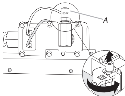
A. Number .0512 LP gas oven bake burner orifice hood
